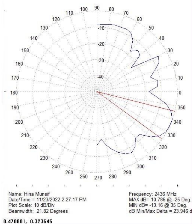
Fig 5: Corrected pattern of double phase shifters malfunctioning.
