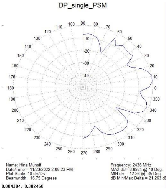
Fig 2: Defected pattern of single phase shifter malfunctioning.
