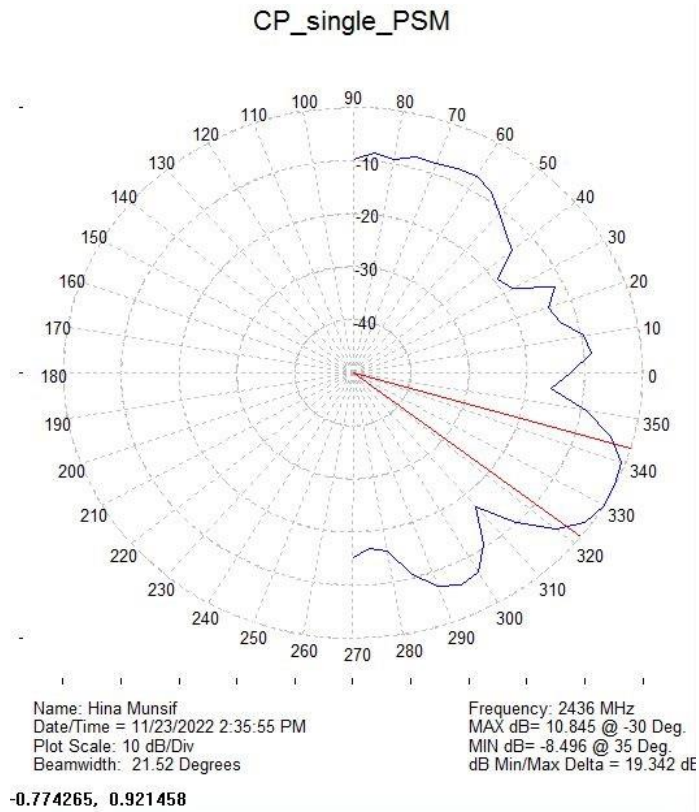
Fig 3: Corrected pattern of single phase shifter malfunctioning.
