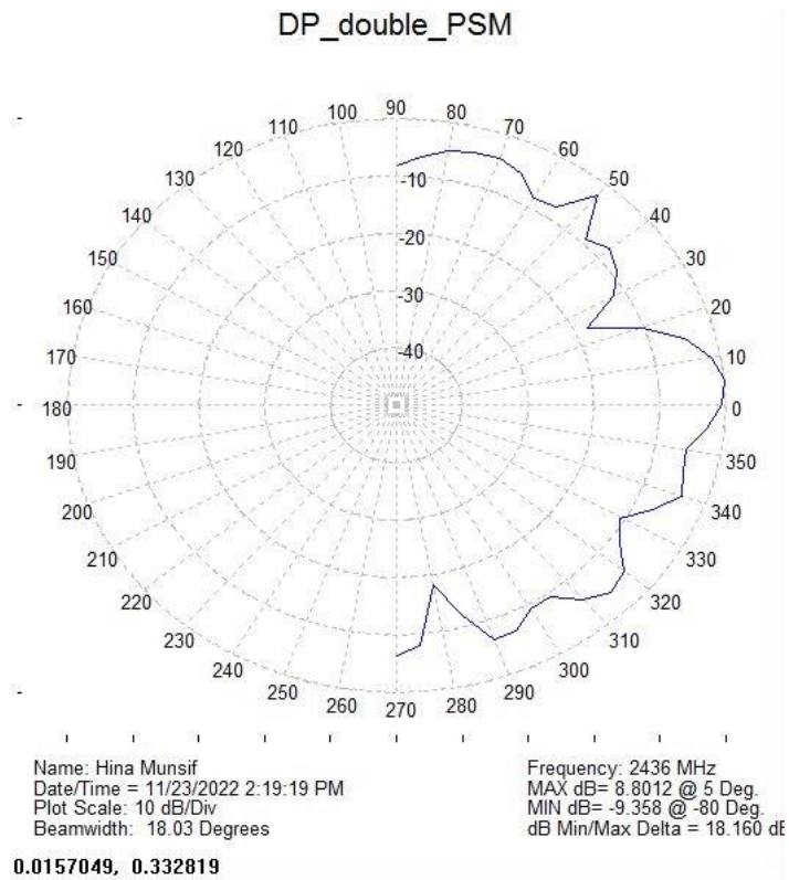
Fig 4: Defected pattern of double phase shifters malfunctioning.
